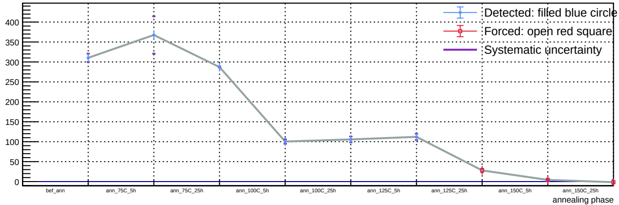
Sensor B1, T = 20\text{ C} , v_{\text{over}} = 5\text{ V} - Spot 4: luminosity vs phase
