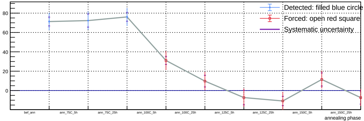
Sensor B1, T = 20\text{ C} , v_{\text{over}} = 5\text{ V} - Spot 41: luminosity vs phase
