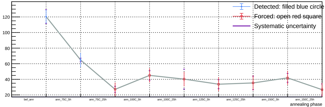
Sensor B1, T = 20\text{ C} , v_{\text{over}} = 5\text{ V} - Spot 44: luminosity vs phase
