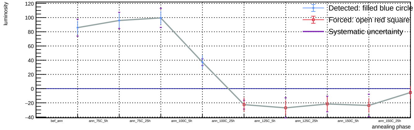
Sensor B1, T = 20\text{ C} , v_{\text{over}} = 5\text{ V} - Spot 49: luminosity vs phase
