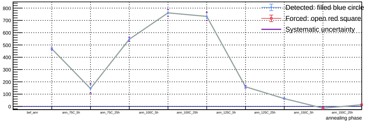
Sensor B1, T = 20\text{ C} , v_{\text{over}} = 5\text{ V} - Spot 5: luminosity vs phase
