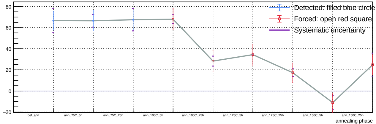
Sensor B1, T = 20\text{ C} , v_{\text{over}} = 5\text{ V} - Spot 50: luminosity vs phase
