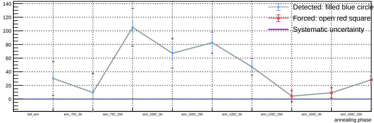
Sensor B1, T = 20\text{ C} , v_{\text{over}} = 5\text{ V} - Spot 54: luminosity vs phase
