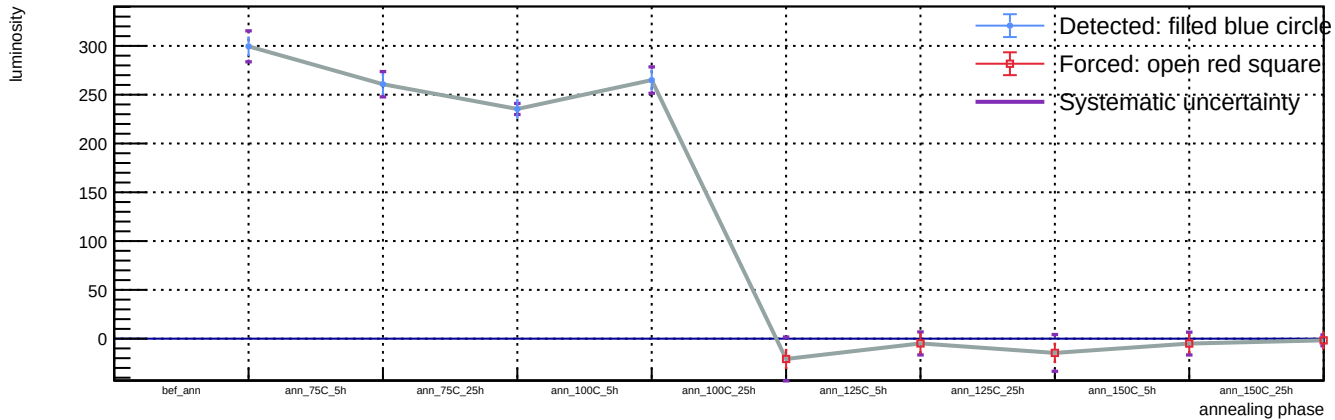
Sensor B1, T = 20\text{ C} , v_{\text{over}} = 5\text{ V} - Spot 56: luminosity vs phase
