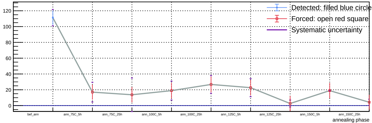
Sensor B1, T = 20\text{ C} , v_{\text{over}} = 5\text{ V} - Spot 57: luminosity vs phase
