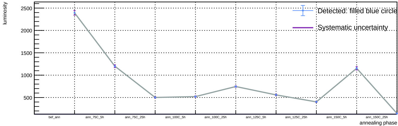
Sensor B1, T = 20\text{ C} , v_{\text{over}} = 5\text{ V} - Spot 60: luminosity vs phase
