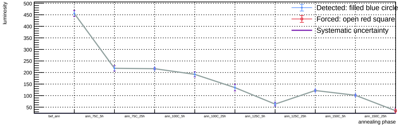
Sensor B1, T = 20\text{ C} , v_{\text{over}} = 5\text{ V} - Spot 61: luminosity vs phase
