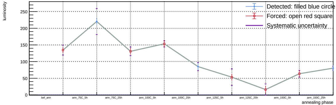
Sensor B1, T = 20\text{ C} , v_{\text{over}} = 5\text{ V} - Spot 64: luminosity vs phase
