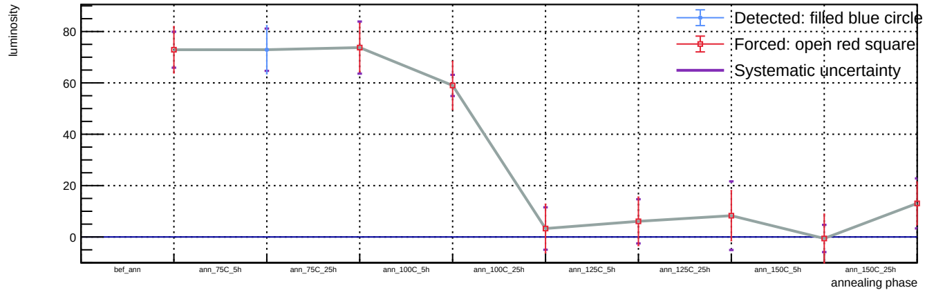
Sensor B1, T = 20\text{ C} , v_{\text{over}} = 5\text{ V} - Spot 66: luminosity vs phase
