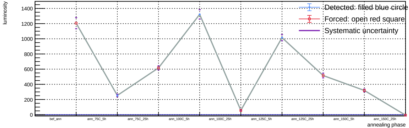
Sensor B1, T = 20\text{ C} , v_{\text{over}} = 5\text{ V} - Spot 70: luminosity vs phase
