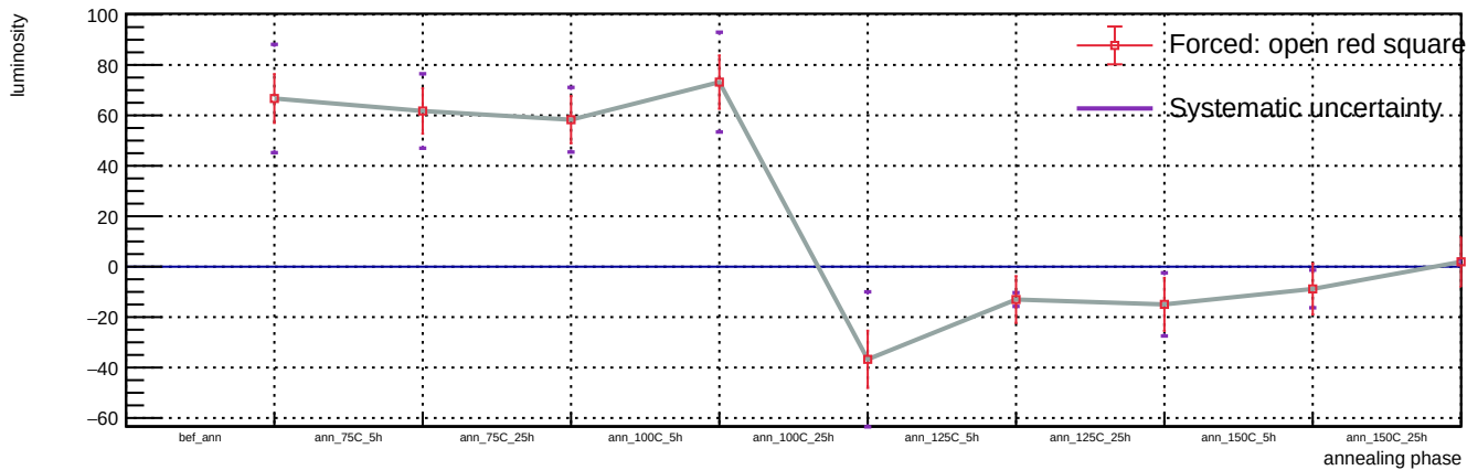
Sensor B1, T = 20\text{ C} , v_{\text{over}} = 5\text{ V} - Spot 73: luminosity vs phase
