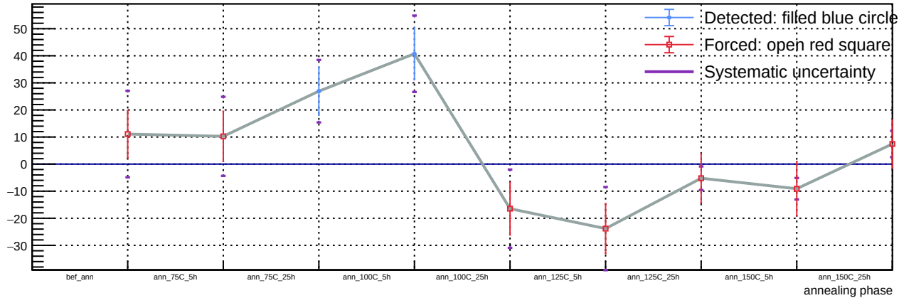
Sensor B1, T = 20\text{ C} , v_{\text{over}} = 5\text{ V} - Spot 75: luminosity vs phase
