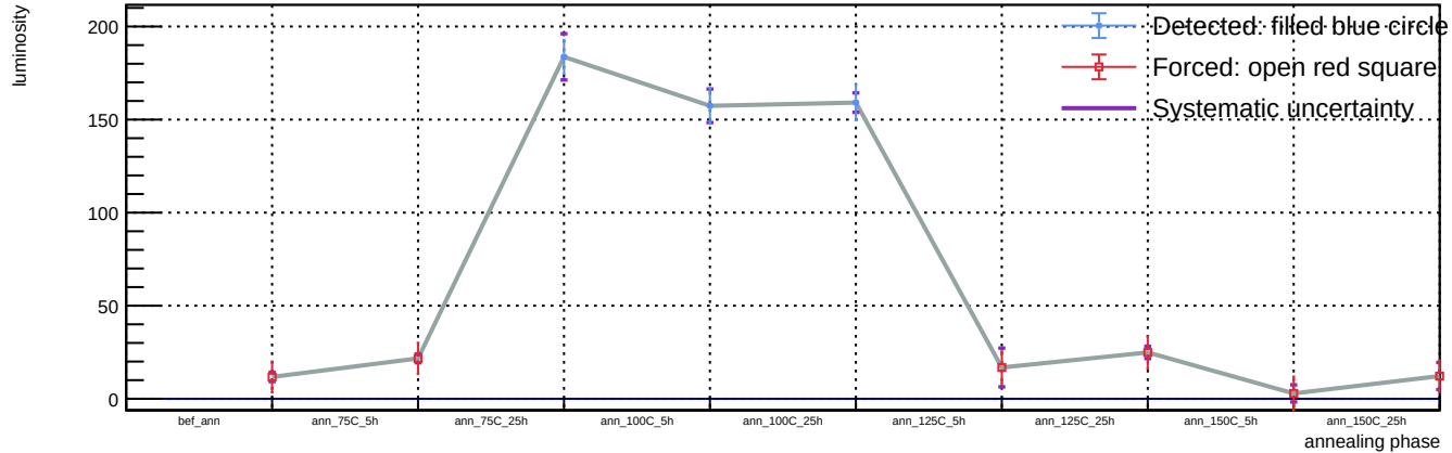
Sensor B1, T = 20\text{ C} , v_{\text{over}} = 5\text{ V} - Spot 76: luminosity vs phase
