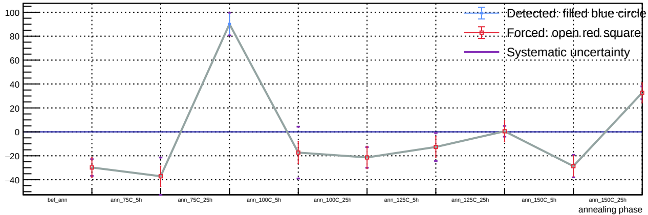
Sensor B1, T = 20\text{ C} , v_{\text{over}} = 5\text{ V} - Spot 77: luminosity vs phase
