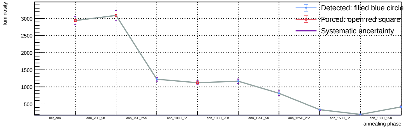
Sensor B1, T = 20\text{ C} , v_{\text{over}} = 5\text{ V} - Spot 78: luminosity vs phase
