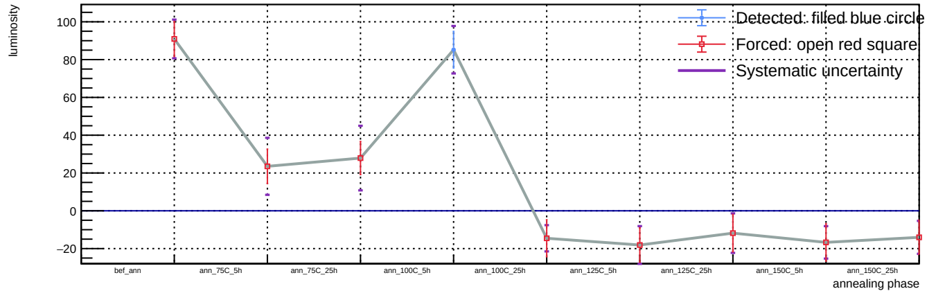
Sensor B1, T = 20\text{ C} , v_{\text{over}} = 5\text{ V} - Spot 81: luminosity vs phase
