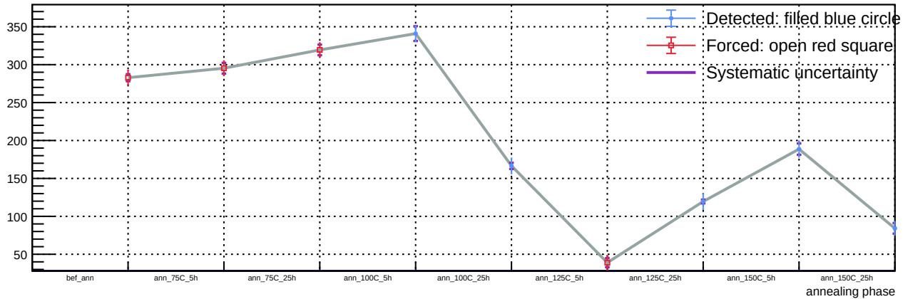
Sensor B1, T = 20\text{ C} , v_{\text{over}} = 5\text{ V} - Spot 83: luminosity vs phase
