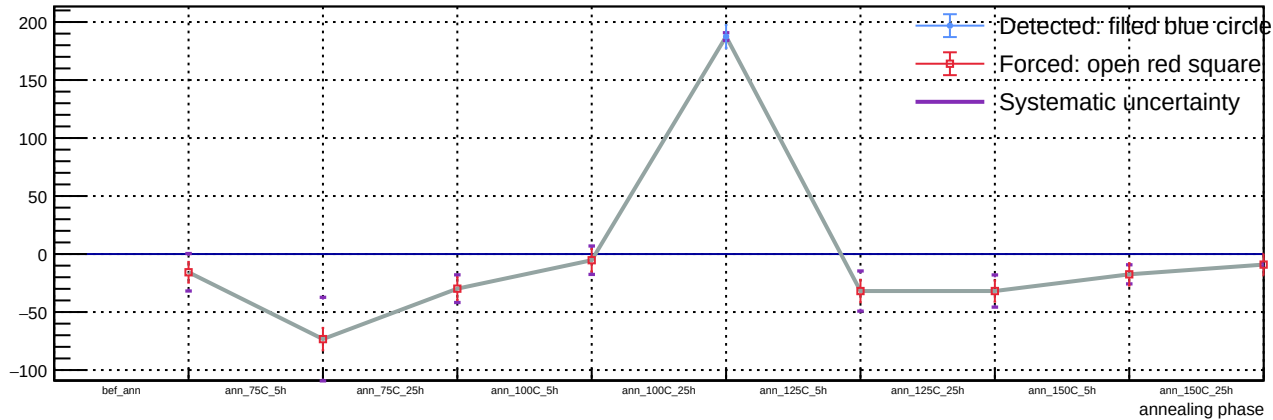
Sensor B1, T = 20\text{ C} , v_{\text{over}} = 5\text{ V} - Spot 86: luminosity vs phase
