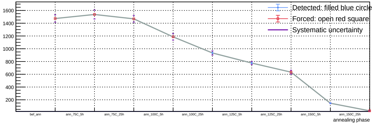
Sensor B1, T = 20\text{ C} , v_{\text{over}} = 5\text{ V} - Spot 90: luminosity vs phase
