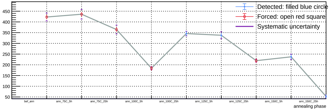
Sensor B1, T = 20\text{ C} , v_{\text{over}} = 5\text{ V} - Spot 91: luminosity vs phase
