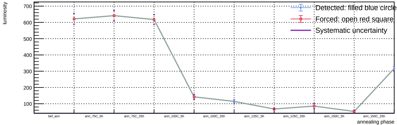
Sensor B1, T = 20\text{ C} , v_{\text{over}} = 5\text{ V} - Spot 93: luminosity vs phase
