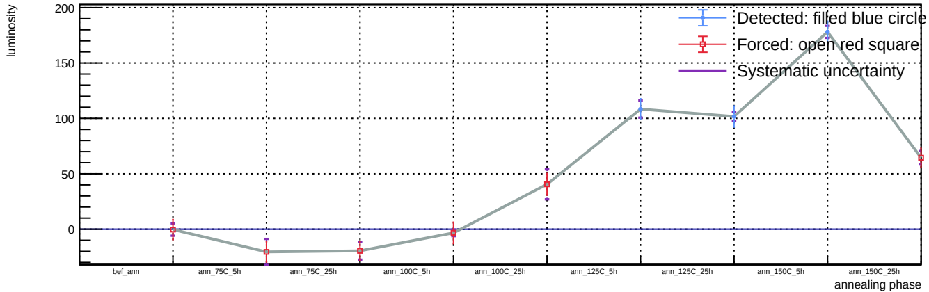
Sensor B1, T = 20\text{ C} , v_{\text{over}} = 5\text{ V} - Spot 98: luminosity vs phase
