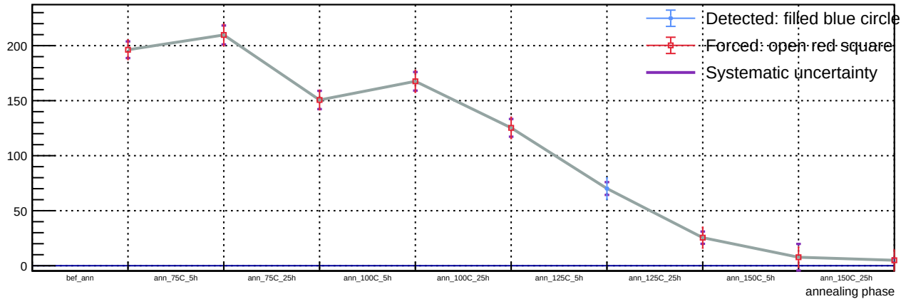
Sensor B1, T = 20\text{ C} , v_{\text{over}} = 5\text{ V} - Spot 99: luminosity vs phase
