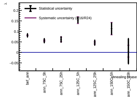
Sensor B1, v = 3 V - Spot 53
