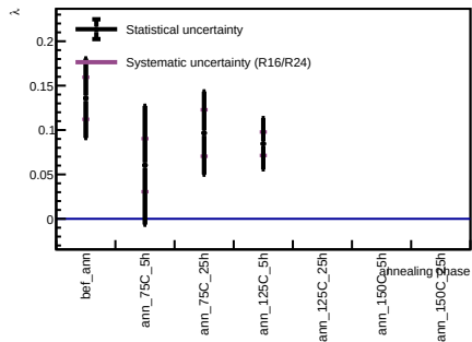
Sensor B1, v = 3 V - Spot 48
