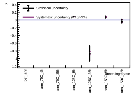
Sensor B1, v = 3 V - Spot 87
