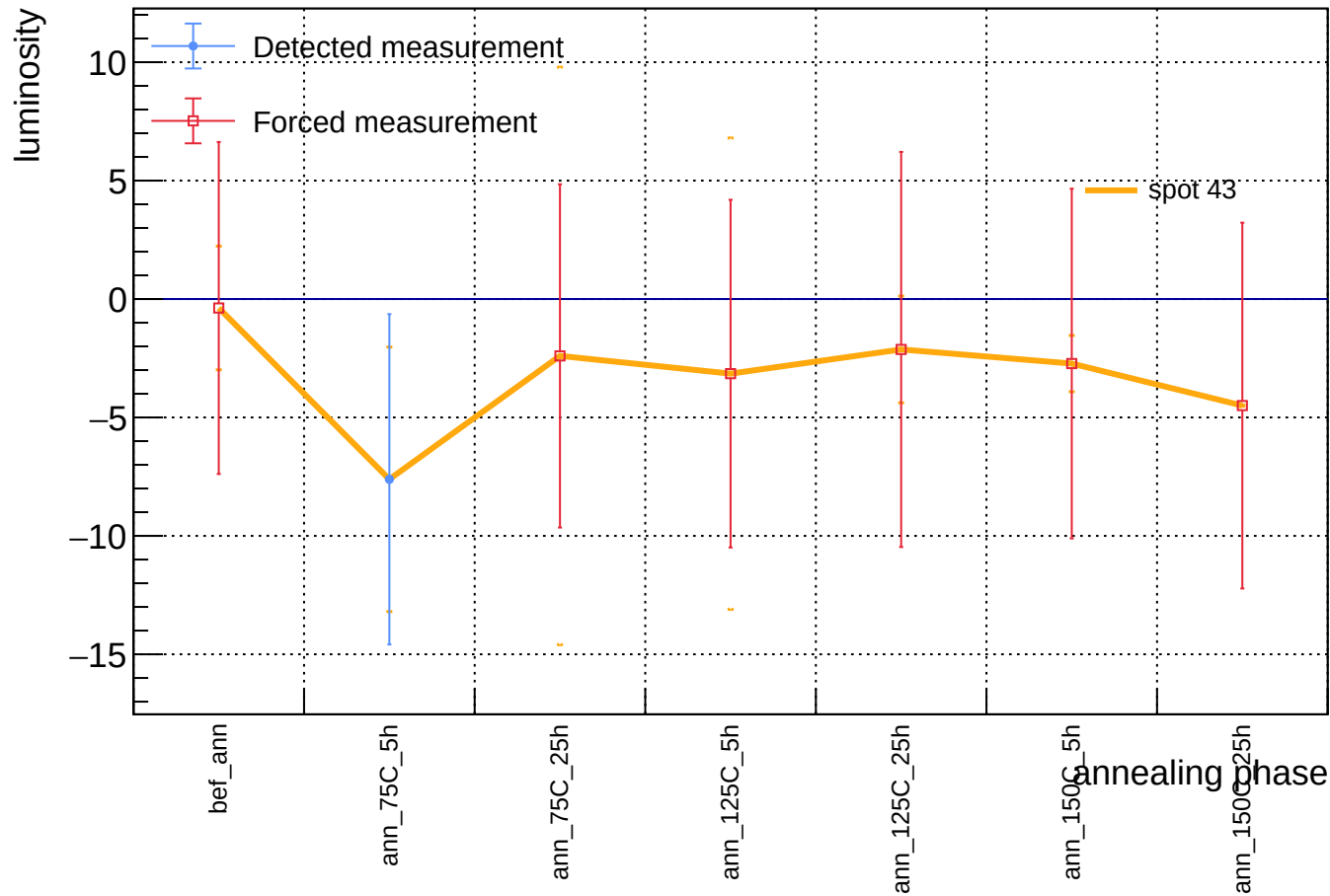
Sensor B1, v = 3 V, T = 23 °C - luminosity vs phase - zero/negative luminosity
