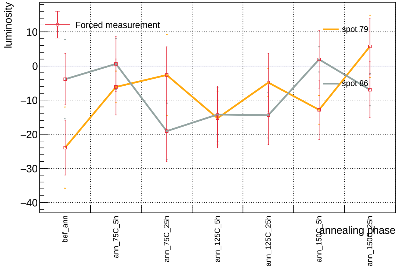
Sensor B1, v = 3 V, T = 23 °C - luminosity vs phase - order 10^0
