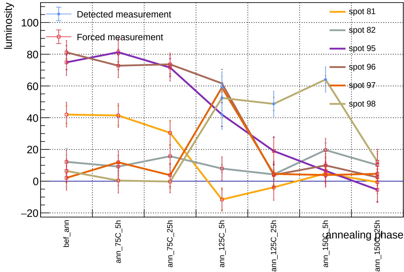
Sensor B1, v = 3 V, T = 23 °C - luminosity vs phase - order 10^1
