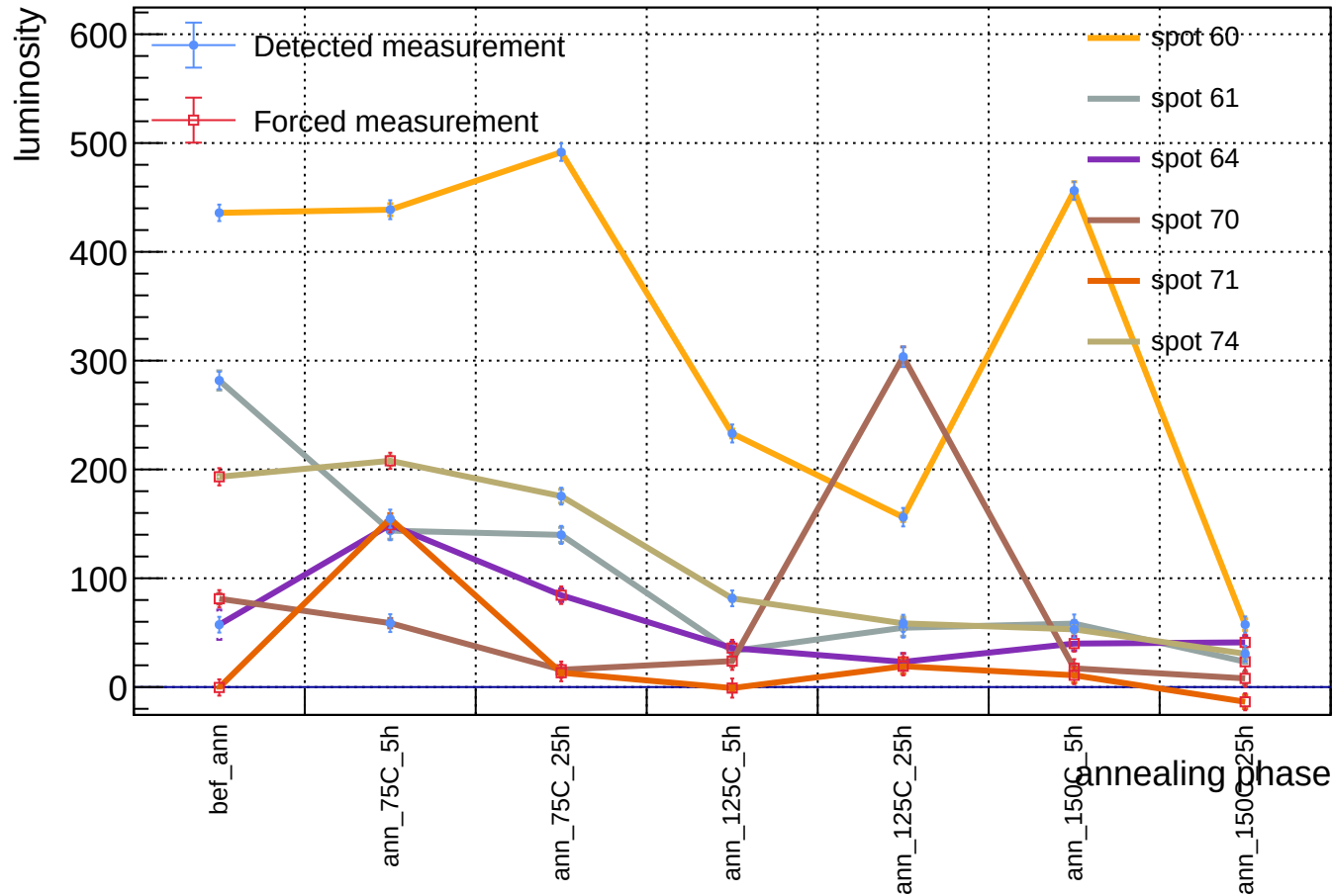
Sensor B1, v = 3 V, T = 23 °C - luminosity vs phase - order 10^2
