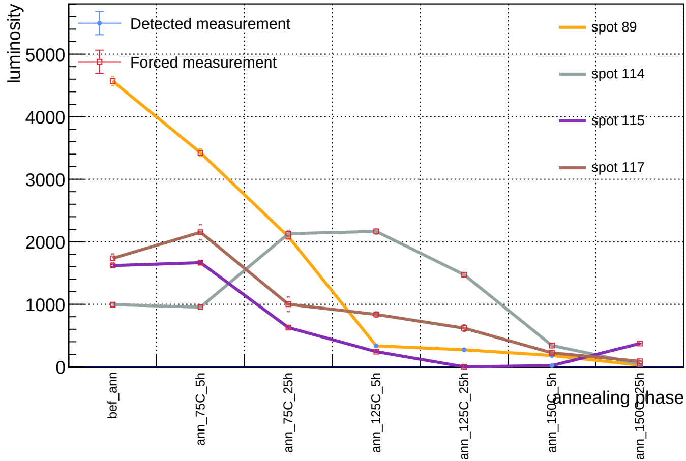
Sensor B1, v = 3 V, T = 23 °C - luminosity vs phase - order 10^3
