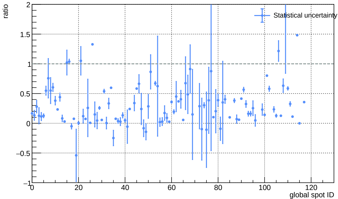
Sensor B1, v = 3 \text{ V} - L(\text{ann\_125C\_25h}) / L(\text{before\_annealing})
