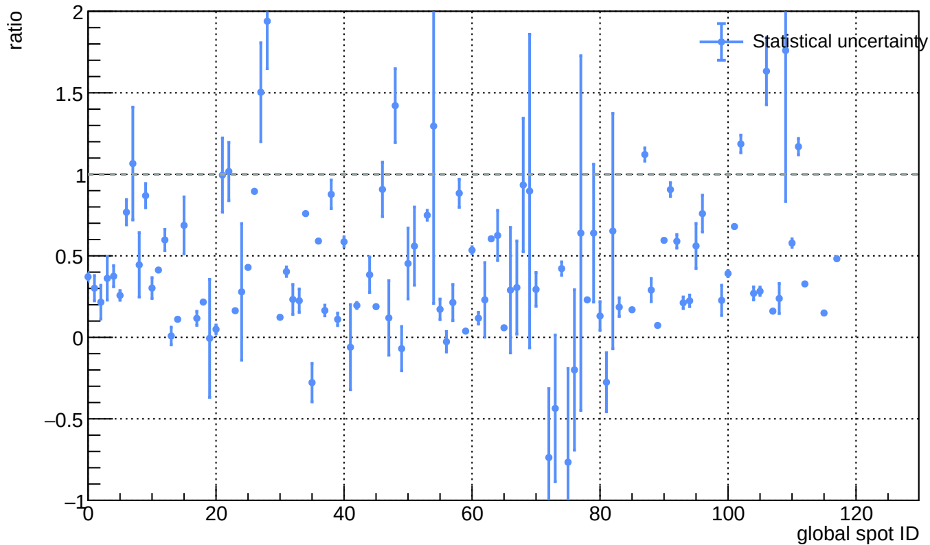
Sensor B1, v = 3\text{ V} - L(\text{ann\_125C\_5h}) / L(\text{before\_annealing})
