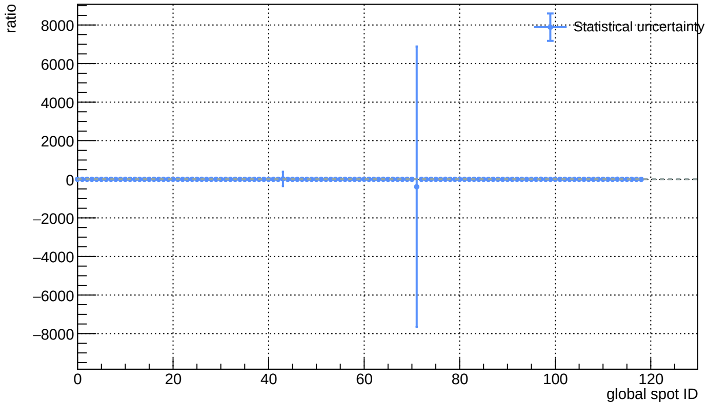
Sensor B1, v = 3 \text{ V} - L(\text{ann\_75C\_5h}) / L(\text{before\_annealing})
