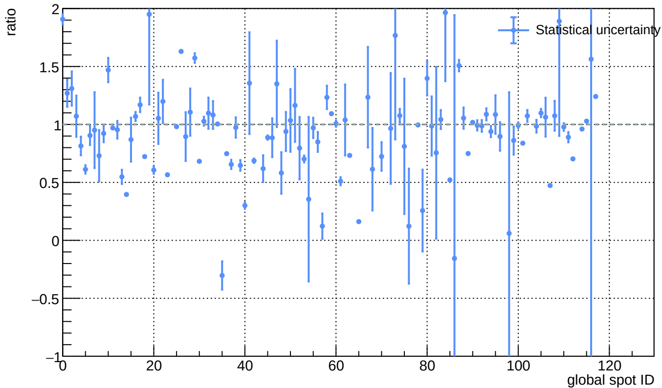
Sensor B1, v = 3 V - L(\text{ann\_75C\_5h}) / L(\text{before\_annealing})
