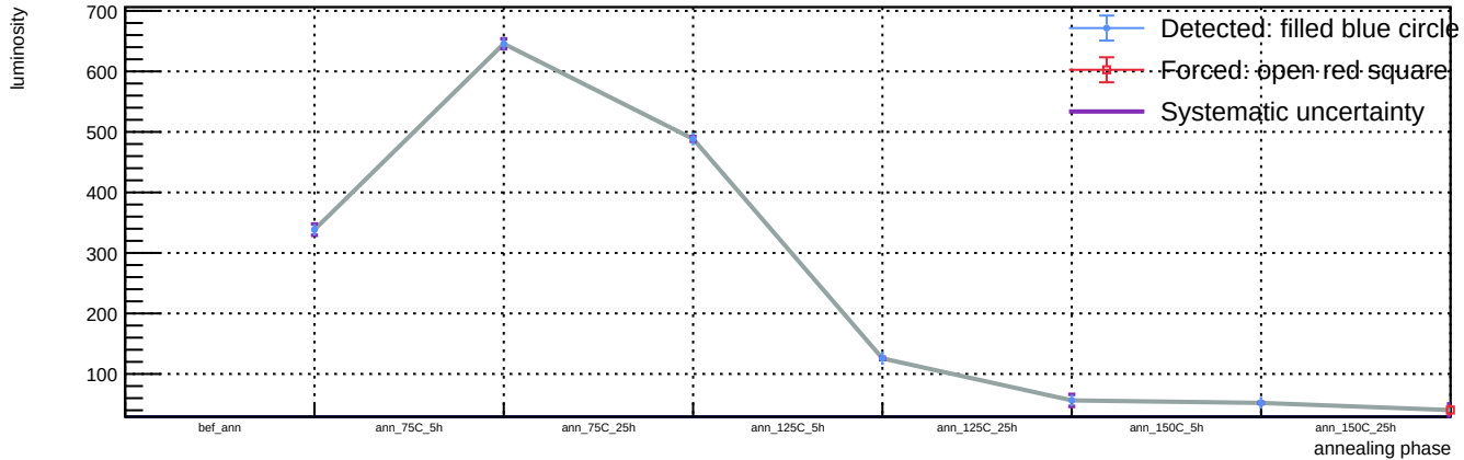
Sensor B1, v = 3 V, T = 23 °C - Spot 0: luminosity vs phase
