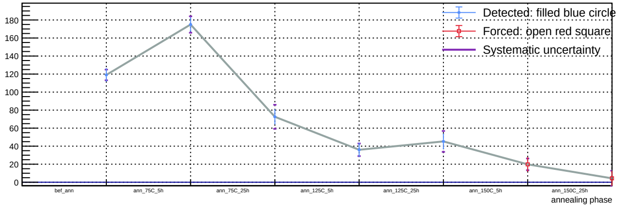
Sensor B1, v = 3 V, T = 23 °C - Spot 10: luminosity vs phase
