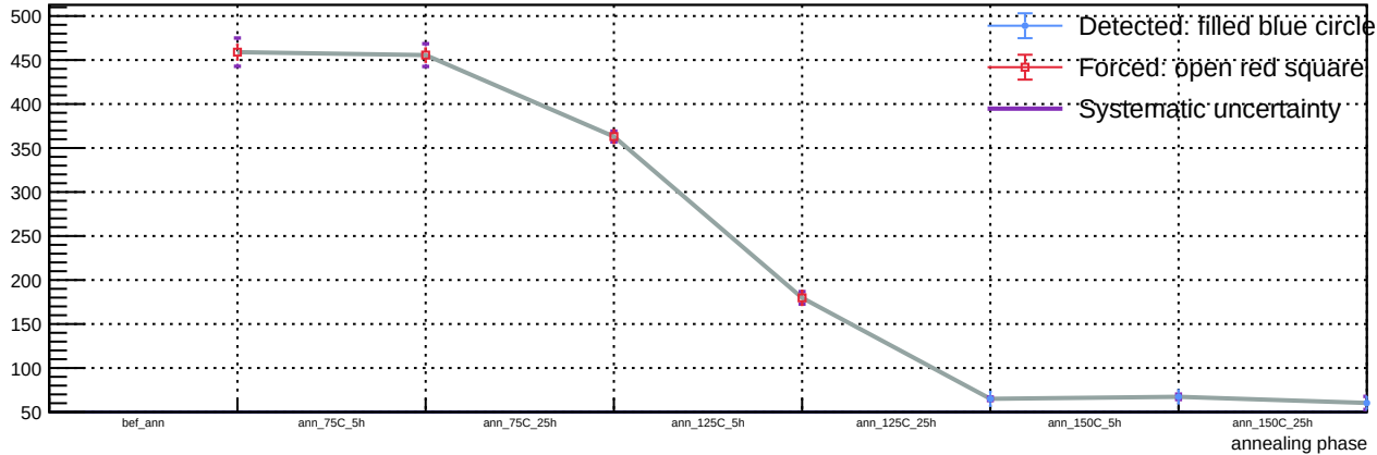
Sensor B1, v = 3 V, T = 23 °C - Spot 100: luminosity vs phase
