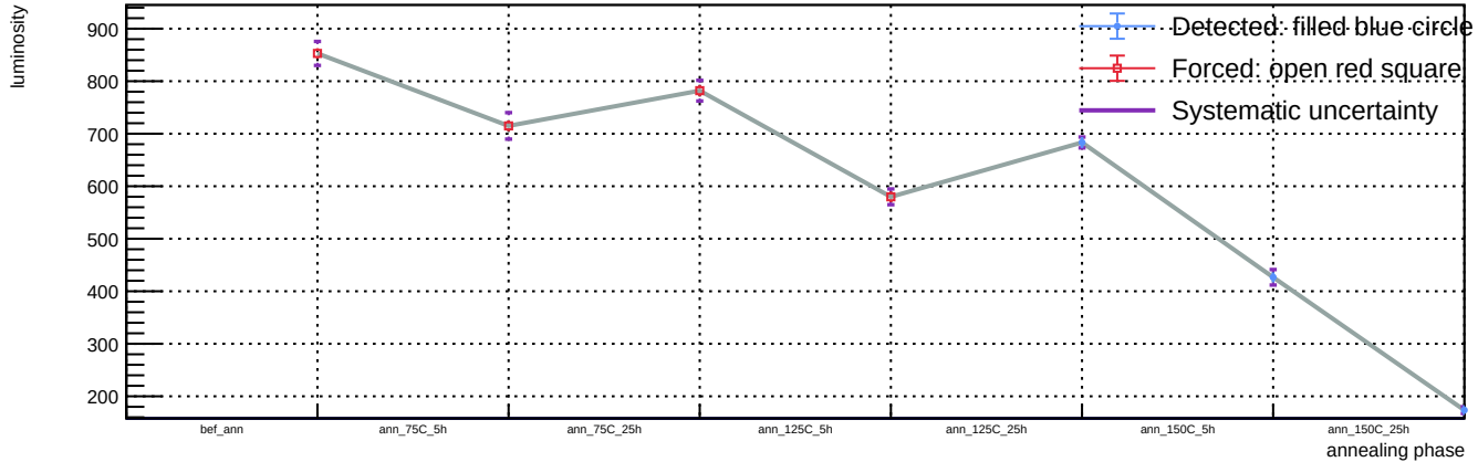
Sensor B1, v = 3 V, T = 23 °C - Spot 101: luminosity vs phase
