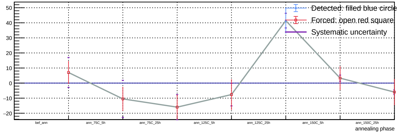
Sensor B1, v = 3 V, T = 23 °C - Spot 103: luminosity vs phase
