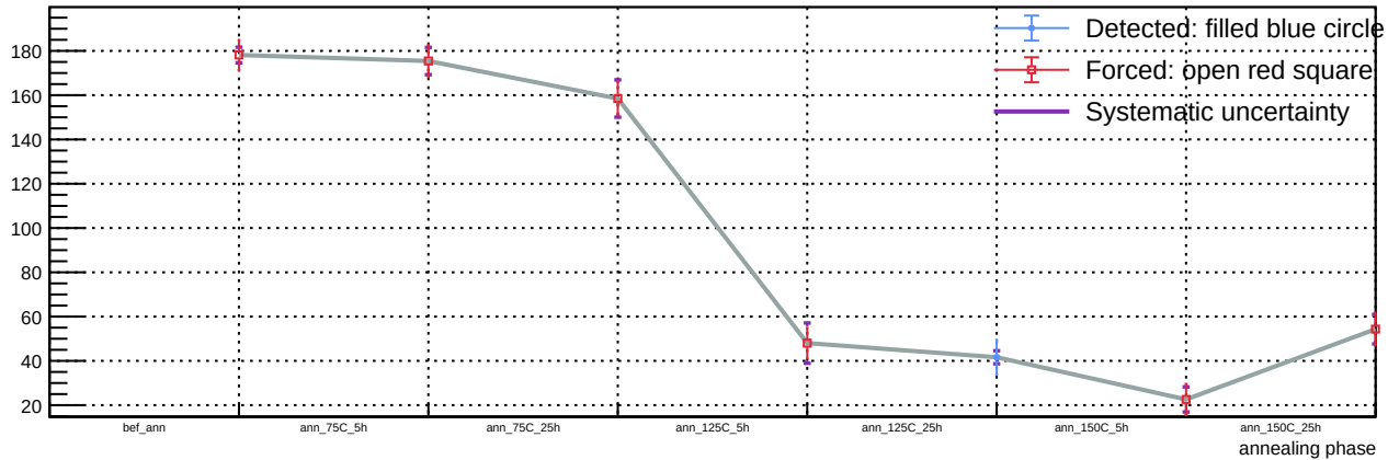
Sensor B1, v = 3 V, T = 23 °C - Spot 104: luminosity vs phase
