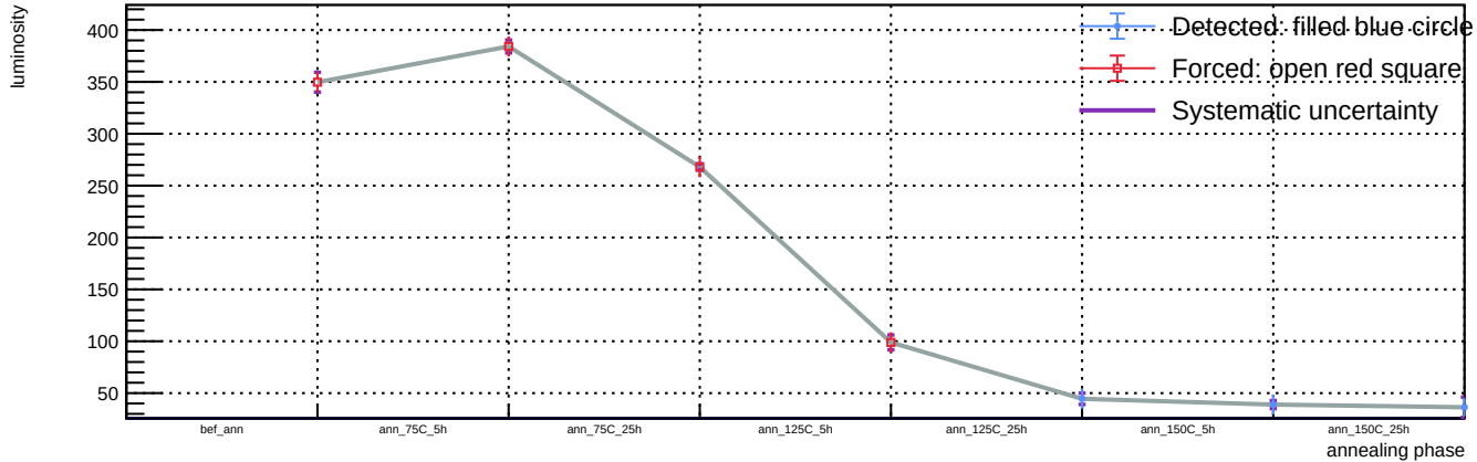
Sensor B1, v = 3 V, T = 23 °C - Spot 105: luminosity vs phase
