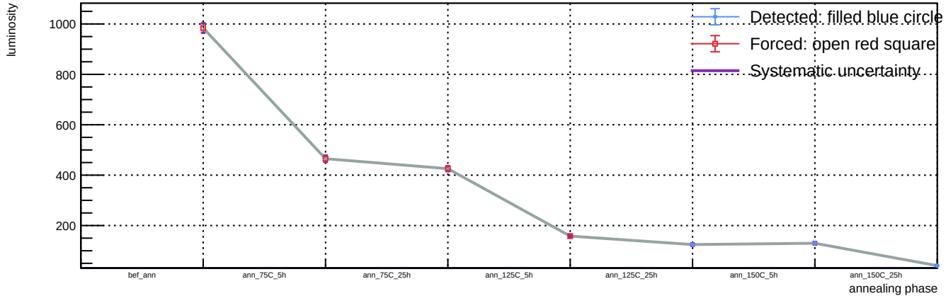
Sensor B1, v = 3 V, T = 23 °C - Spot 107: luminosity vs phase
