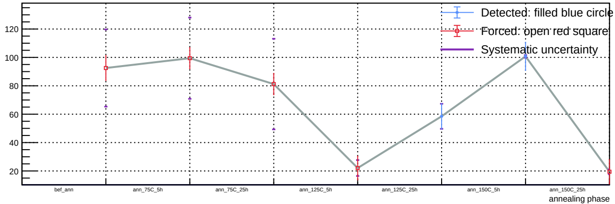
Sensor B1, v = 3 V, T = 23 °C - Spot 108: luminosity vs phase
