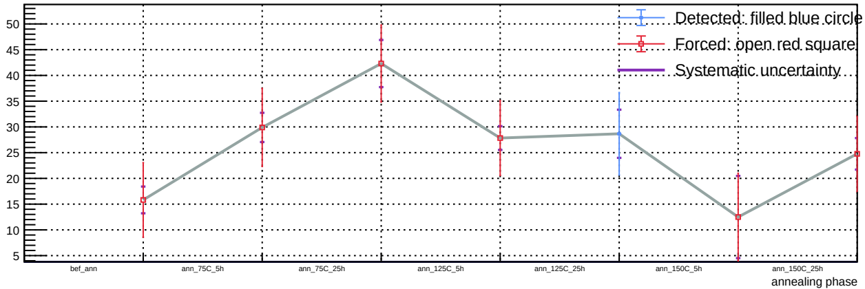
Sensor B1, v = 3 V, T = 23 °C - Spot 109: luminosity vs phase
