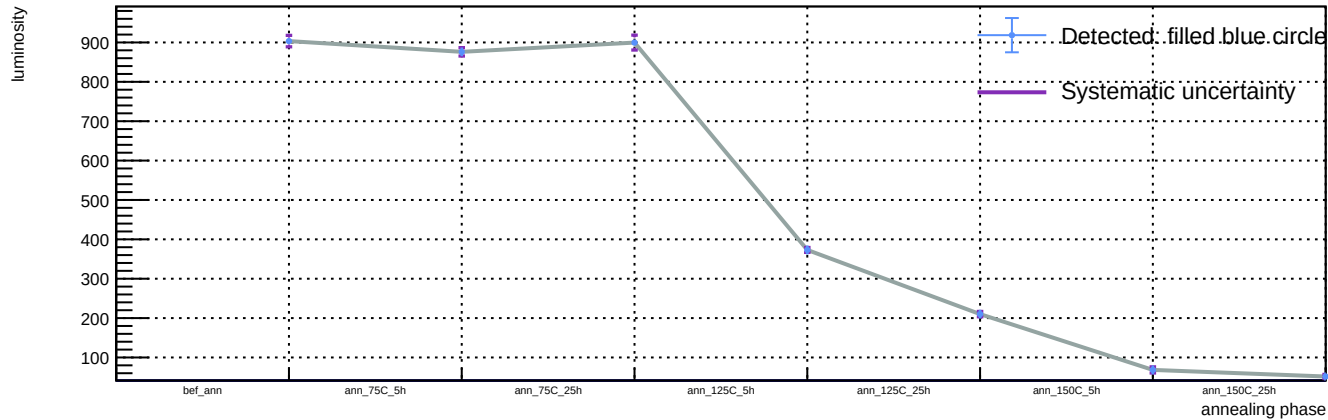
Sensor B1, v = 3 \text{ V} , T = 23 \text{ }^{\circ}\text{C} - Spot 11: luminosity vs phase
