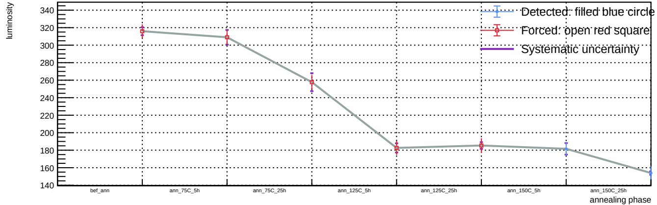
Sensor B1, v = 3 V, T = 23 °C - Spot 110: luminosity vs phase
